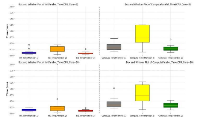
Figure 12: Comparison between initialization time (InitParallel_Time) and computation time (iComputeParallel_Time) for CPU core 8 & 10 configurations across multiple PCs.
