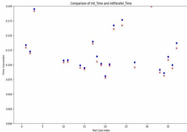
Figure 9: compares the initialization performance between standard and parallel methods for each test case.
