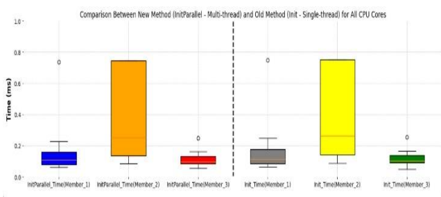
Figure 17: Performance Comparison of both the new multi-threaded method (InitParallel) and the old single-threaded method (Init) across 16 CPU Cores.
