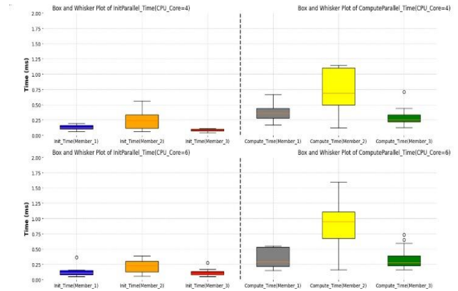
Figure 11: Comparison between initialization time (InitParallel_Time) and computation time (iComputeParallel_Time) for CPU core 4 & 6 configurations across multiple PCs.
