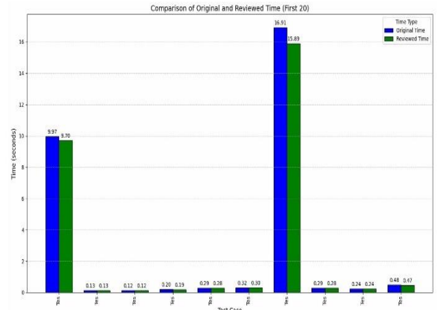
Figure 7: Comparison of Original and Reviewed Time for each test case (First 20).
